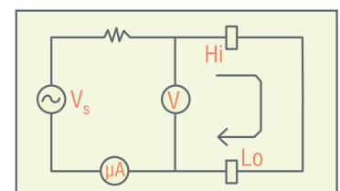
Figure 4.3 : Short Circuit C_m \gg C_x
