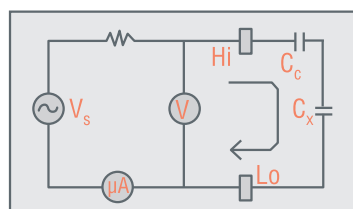
Figure 4.2 : Open Circuit C_m = C_c * C_x / (C_c + C_x) \ll C_x
