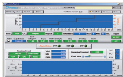
Program Sequence Function
