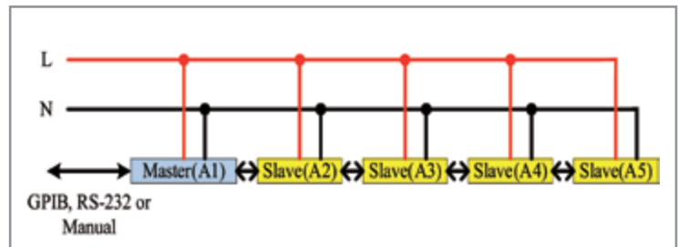
Figure 10: Parallel connection
