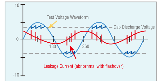
Flashover Waveform
