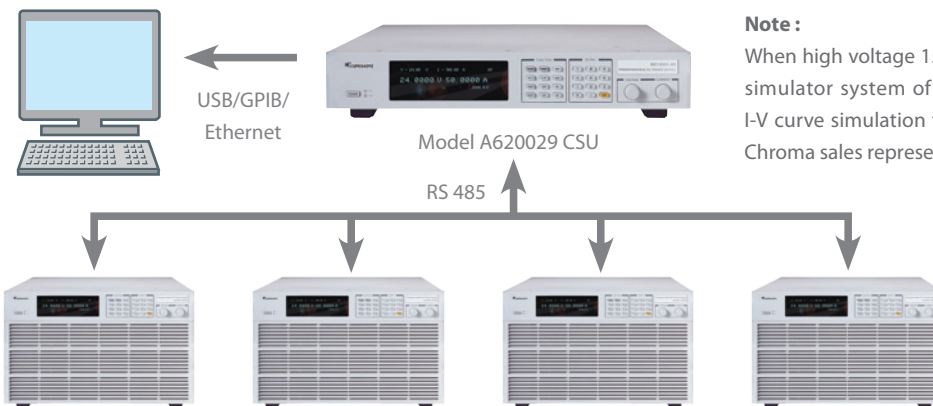
1500V/60A/90kW output Solar Array Simulator
