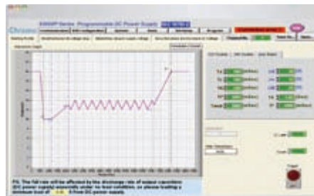
ISO 16750-2 4.5.3 Starting Profile
