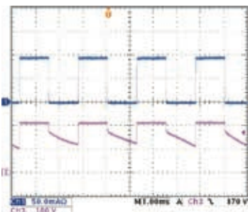
Figure 2 - LED dimming test
