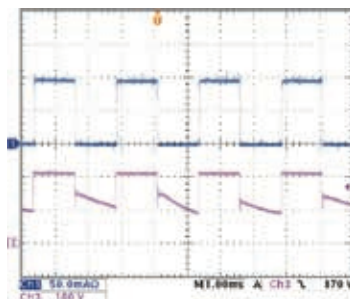
Figure 3 - 63110A dimming test
