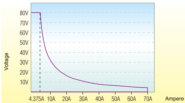
Model 63123A Input Characteristics
