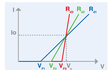
Figure 5 - Simulate different characteristic of LEDs
