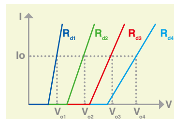
Figure 4 - Simulate different number of LEDs
