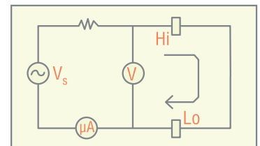
Figure 3.3 : If circuit shorted : C_m \gg C_x
