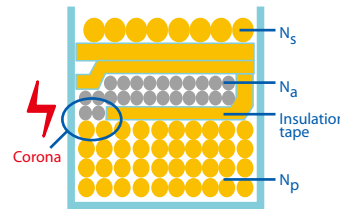
Figure 7.1: Corona
