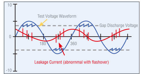
Figure 2: Flashover Waveform
