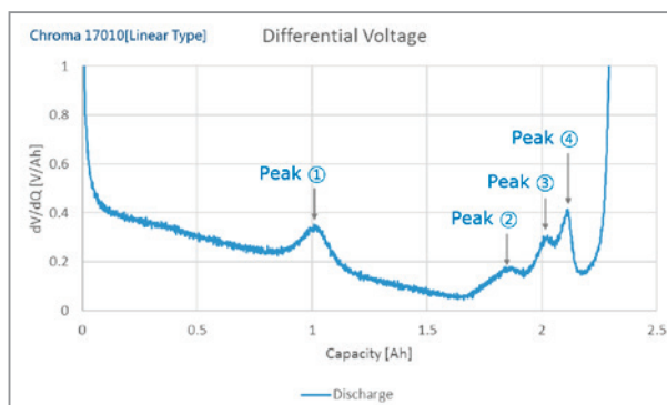
Differential Voltage Analysis Curve
